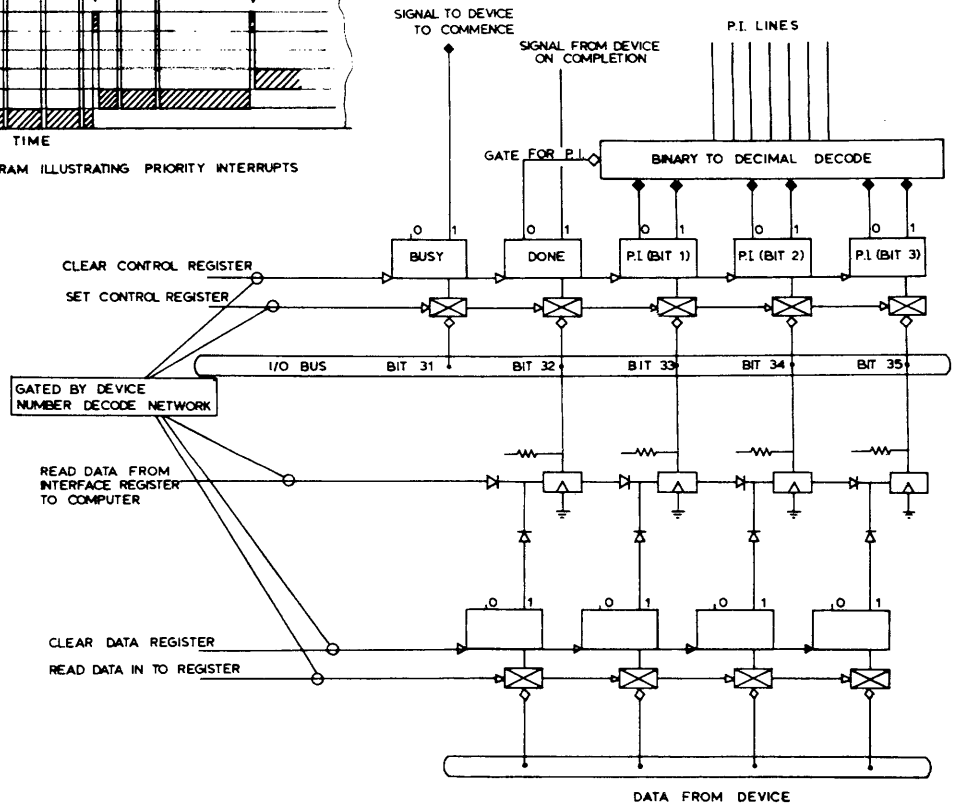
FIGURE 2: SIMPLIFIED LOGIC DIAGRAM SHOWING TYPICAL ARRANGEMENTS OF CONTROL AND DATA REGISTERS
