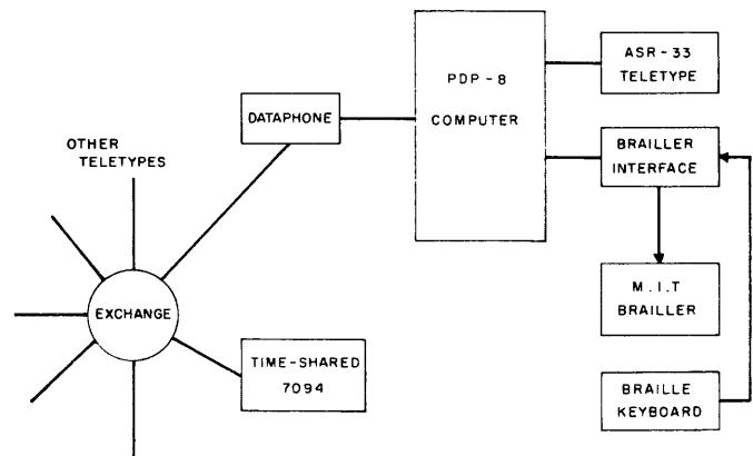
Figure 3 Block Diagram of Braille Translation System
