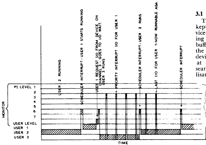
FIGURE 1: SIMPLIFIED DIAGRAM ILLUSTRATING PRIORITY INTERRUPTS
