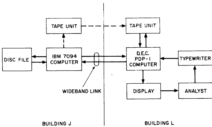
Figure 1 Block Diagram Experimental On-Line System
